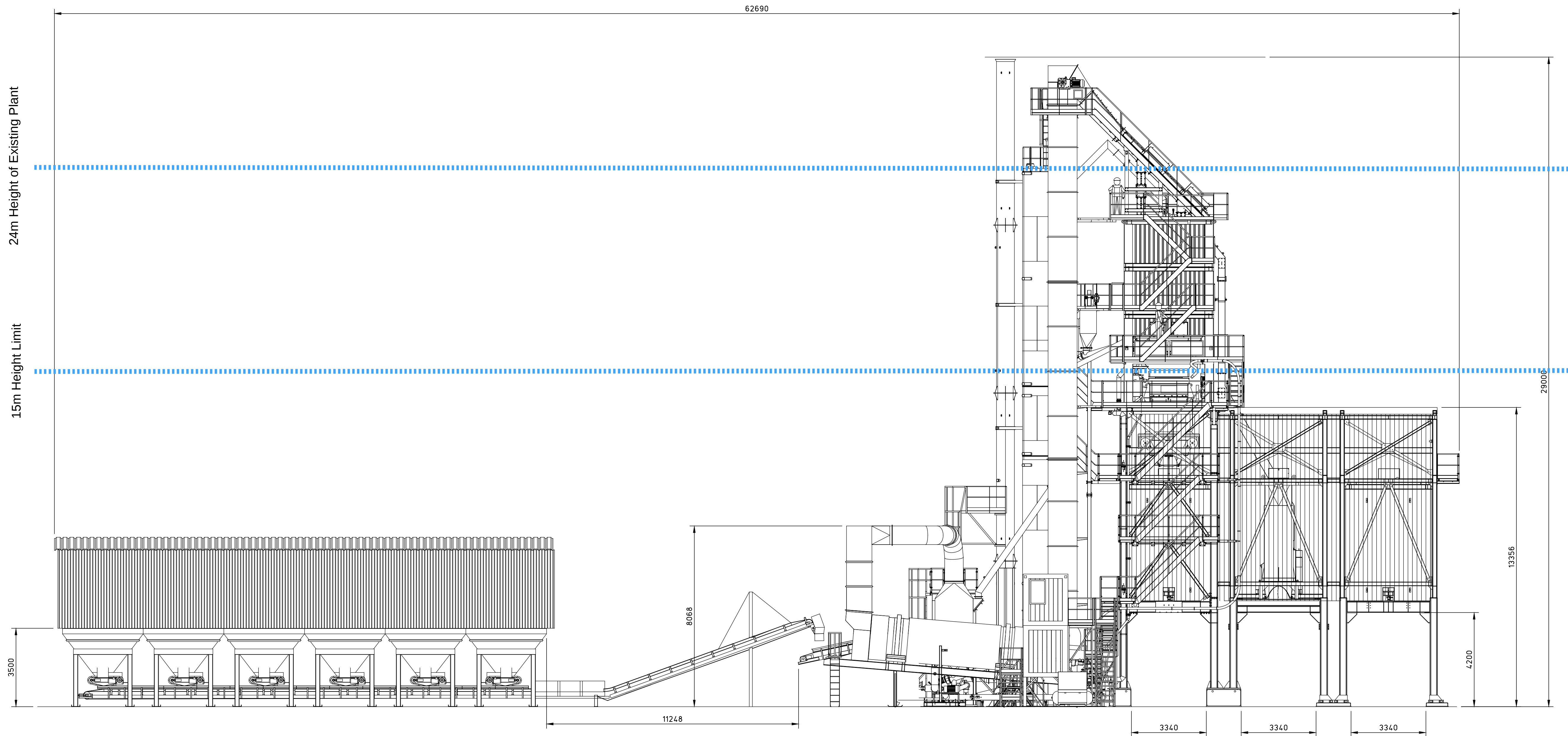
PROPOSED PLANT ELEVATION SCALE 1:100
